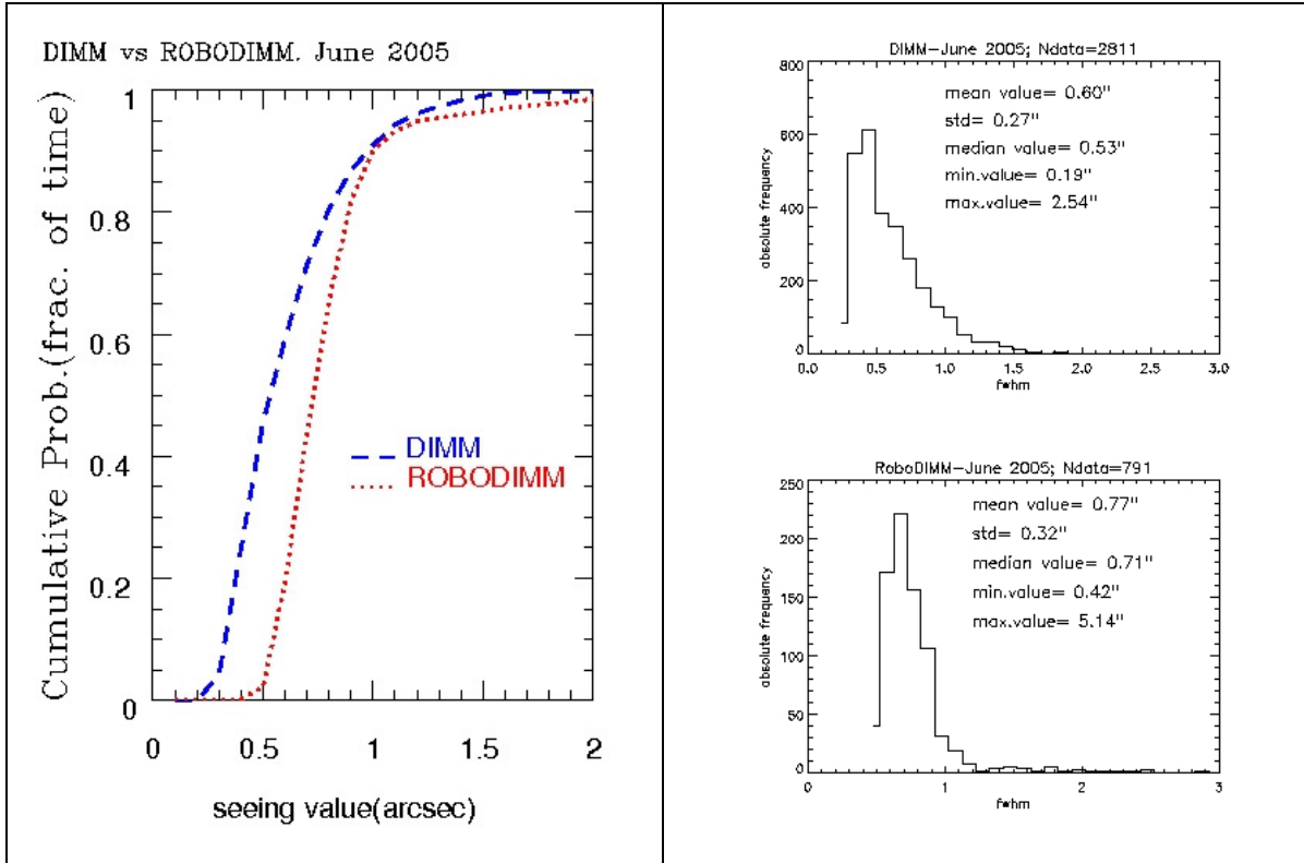
Figure 3b. Cumulative frequency (left) and statistical distribution (right) of the seeing data gathered by the DIMM and RoboDIMM for all common nights in June 2005.
