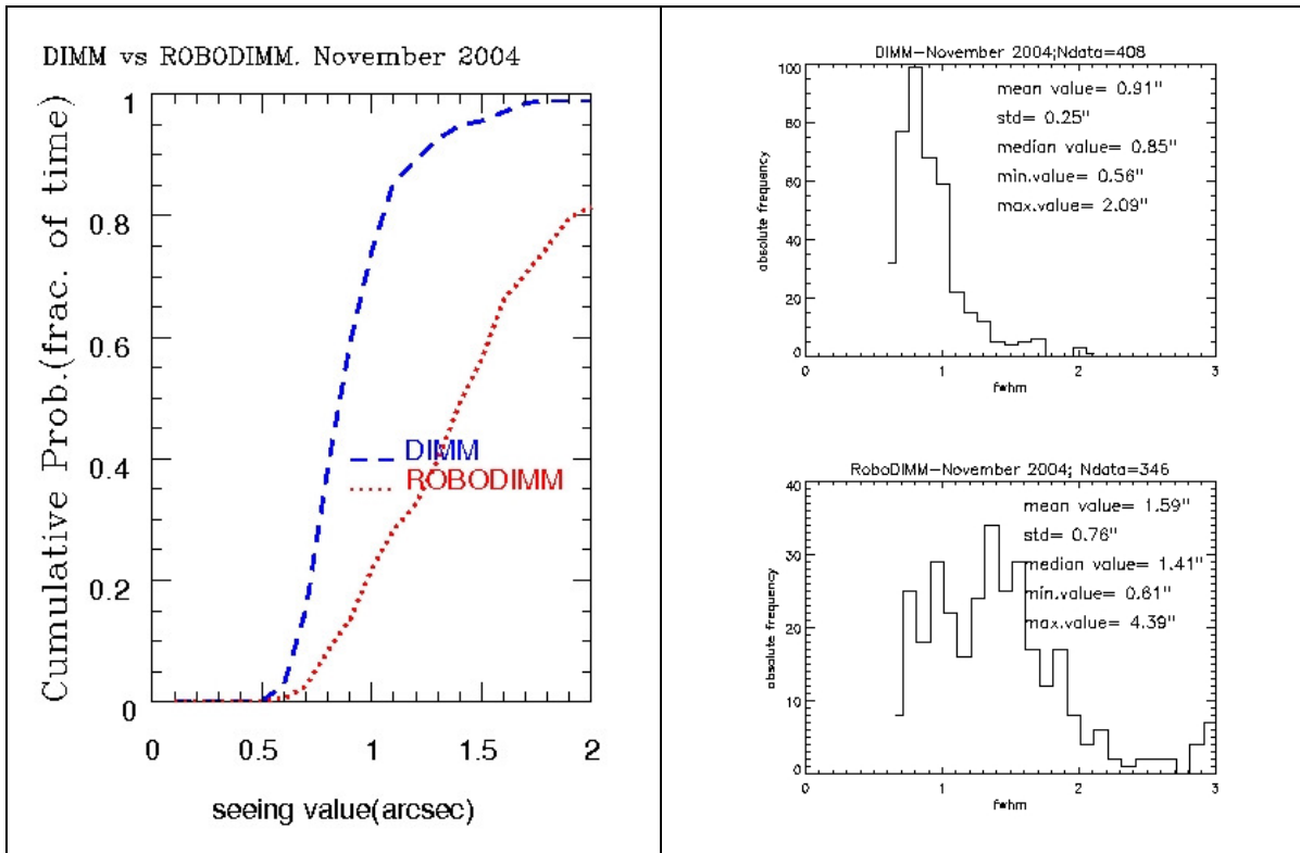
Figure 3a. Cumulative frequency (left) and statistical distribution (right) of the seeing data gathered by the DIMM and RoboDIMM for all possible common nights in November 2004.
