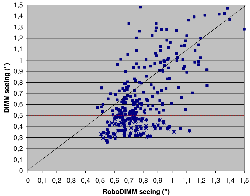
Figure 4. Simultaneous and synchronized seeing values measured by the DIMM and RoboDIMM for several nights (10, 15 and 16 May 2005). Dashed lines mark the RoboDIMM seeing truncation at 0.5". Star points correspond to DIMM points better than 0.5".
