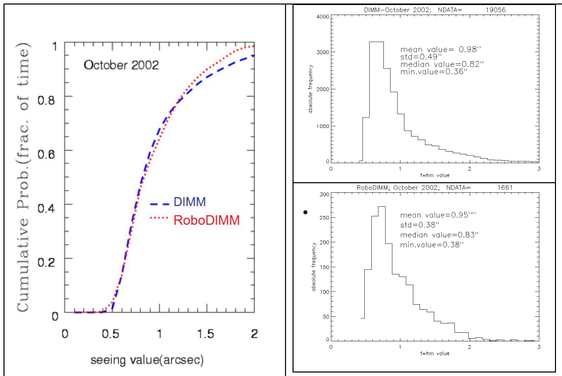
Figure 2. Cumulative frequency (left) and statistical distribution (right) of the simultaneous in time seeing data gathered by the DIMM and RoboDIMM in October 2002.
